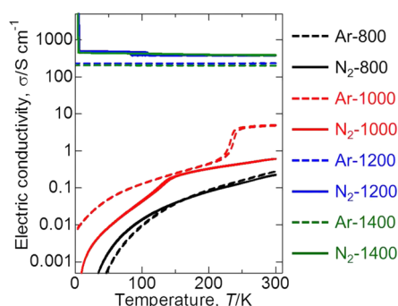
Figure 7. Temperature–electric conductivity relationship of the monolithic samples calcined at different temperatures under Ar and N 2 atmospheres. The broken and solid curves are for the samples treated under Ar and N 2 atmospheres, respectively.
